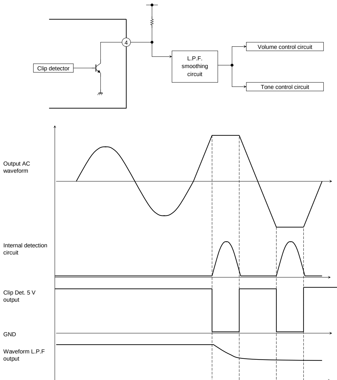
Figure 3 Clip Detection
