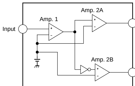
Figure 1 Block Diagram
